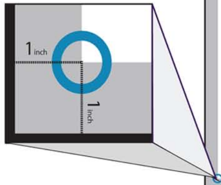
Grommet Placement
